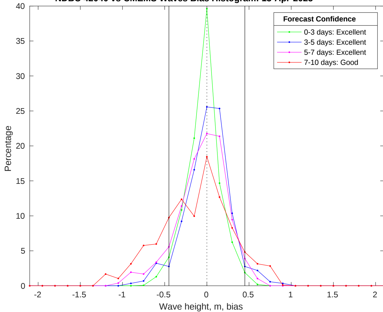
NDBC 42040 vs CMEMS Waves Bias Histogram: 13-Apr-2025
