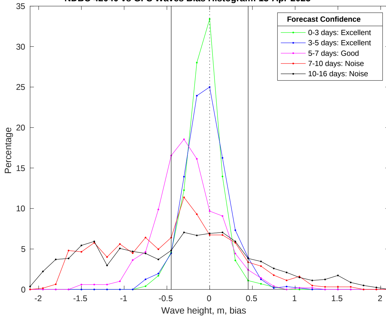
NDBC 42040 vs GFS Waves Bias Histogram: 13-Apr-2025
