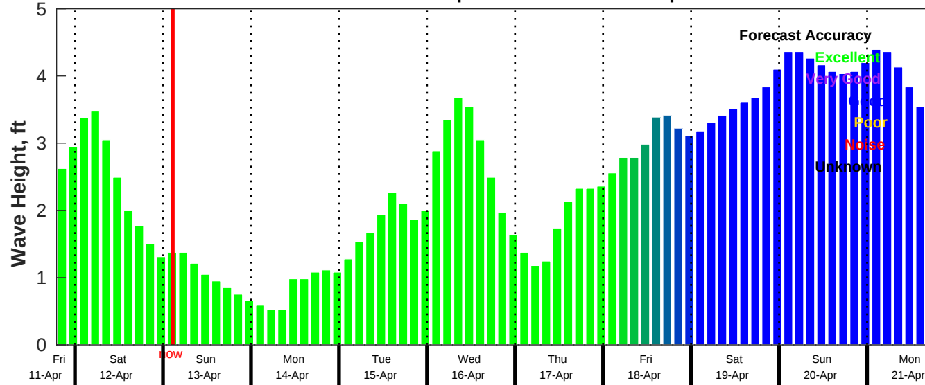
CMEMS Wave Forecast for NDBC 42040 from 11-Apr-2025 19:00:00 to 21-Apr-2025 19:00:00
