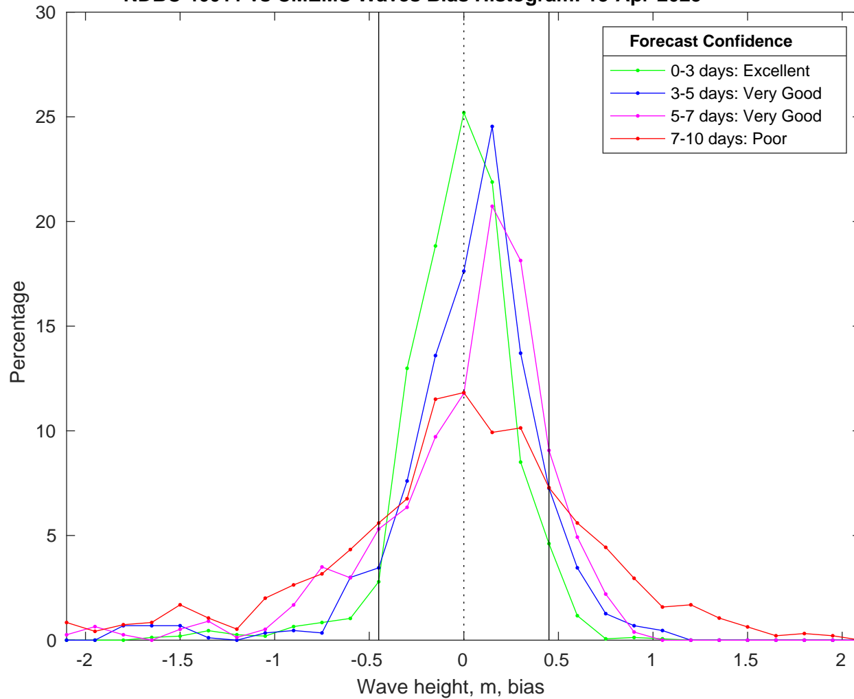
NDBC 46011 vs CMEMS Waves Bias Histogram: 13-Apr-2025
