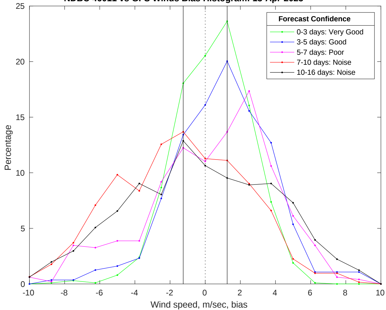
NDBC 46011 vs GFS Winds Bias Histogram: 13-Apr-2025
