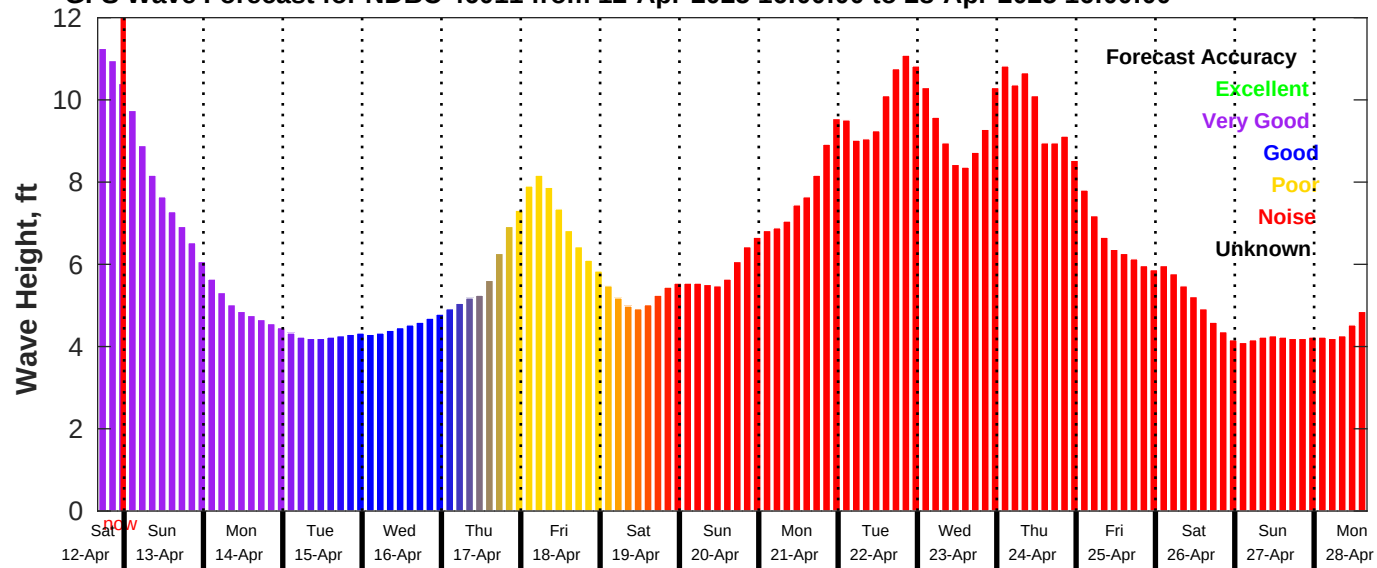
GFS Wave Forecast for NDBC 46011 from 12-Apr-2025 16:00:00 to 28-Apr-2025 16:00:00
