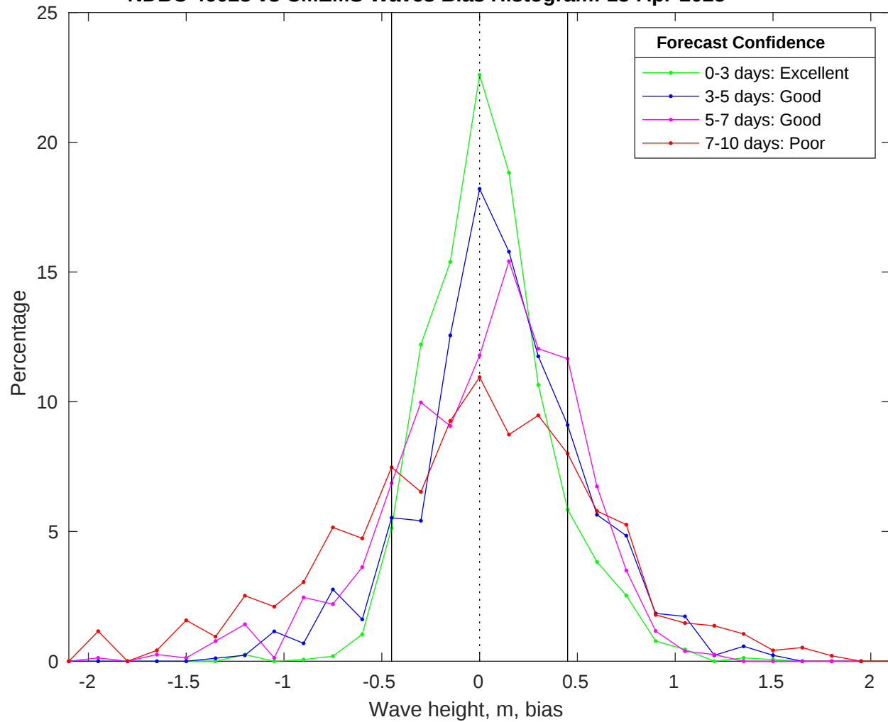
NDBC 46028 vs CMEMS Waves Bias Histogram: 13-Apr-2025
