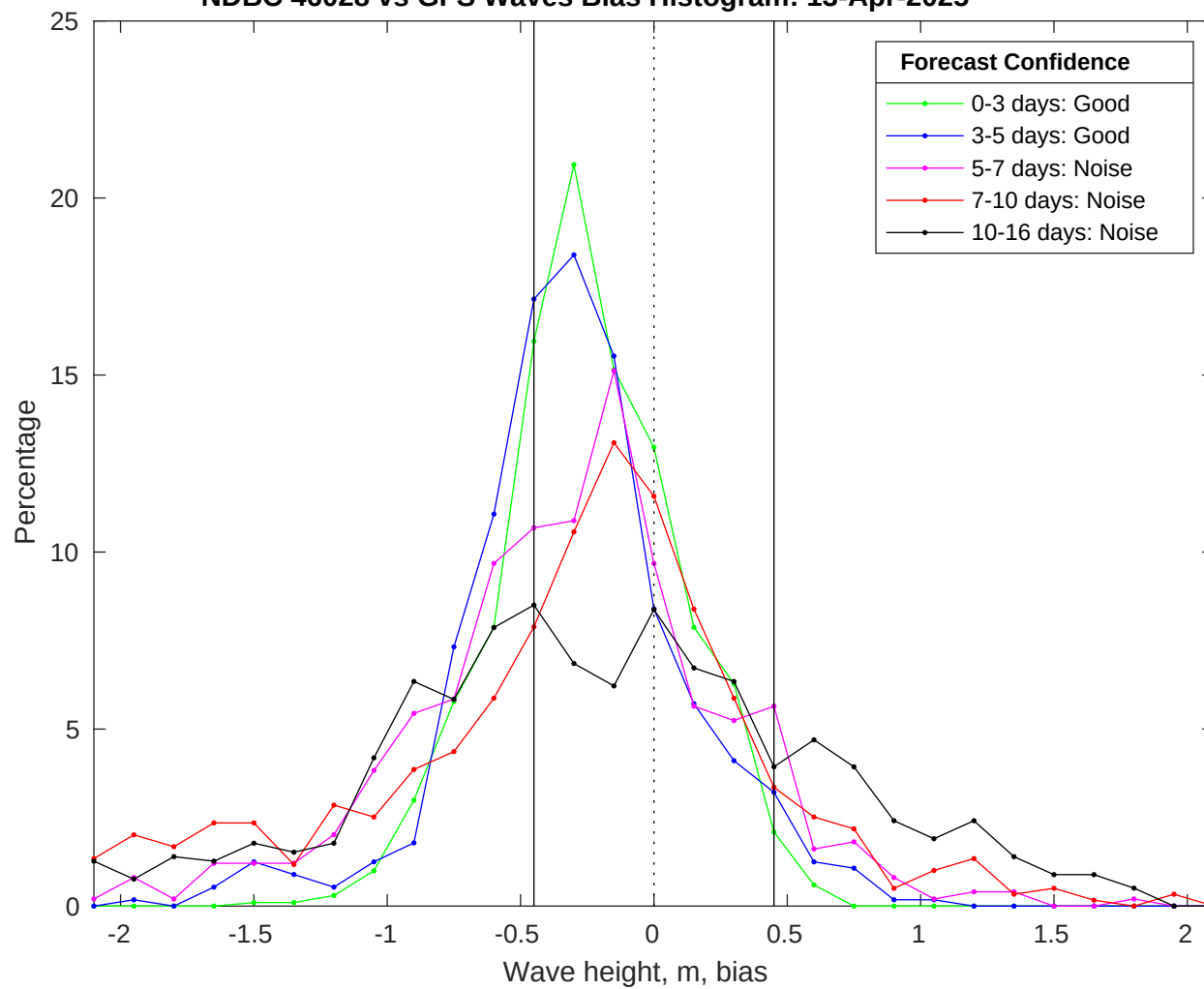
NDBC 46028 vs GFS Waves Bias Histogram: 13-Apr-2025
