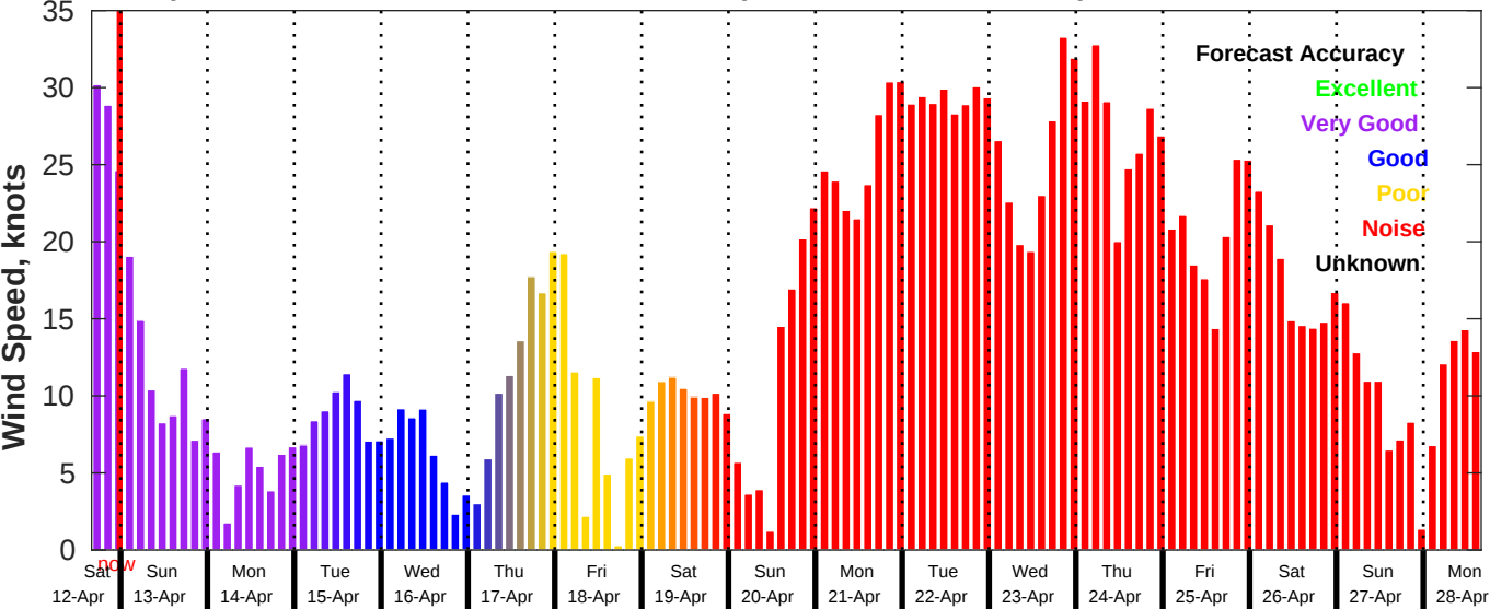
GFS Wind Speed Forecast for NDBC 46028 from 12-Apr-2025 16:00:00 to 28-Apr-2025 16:00:00
