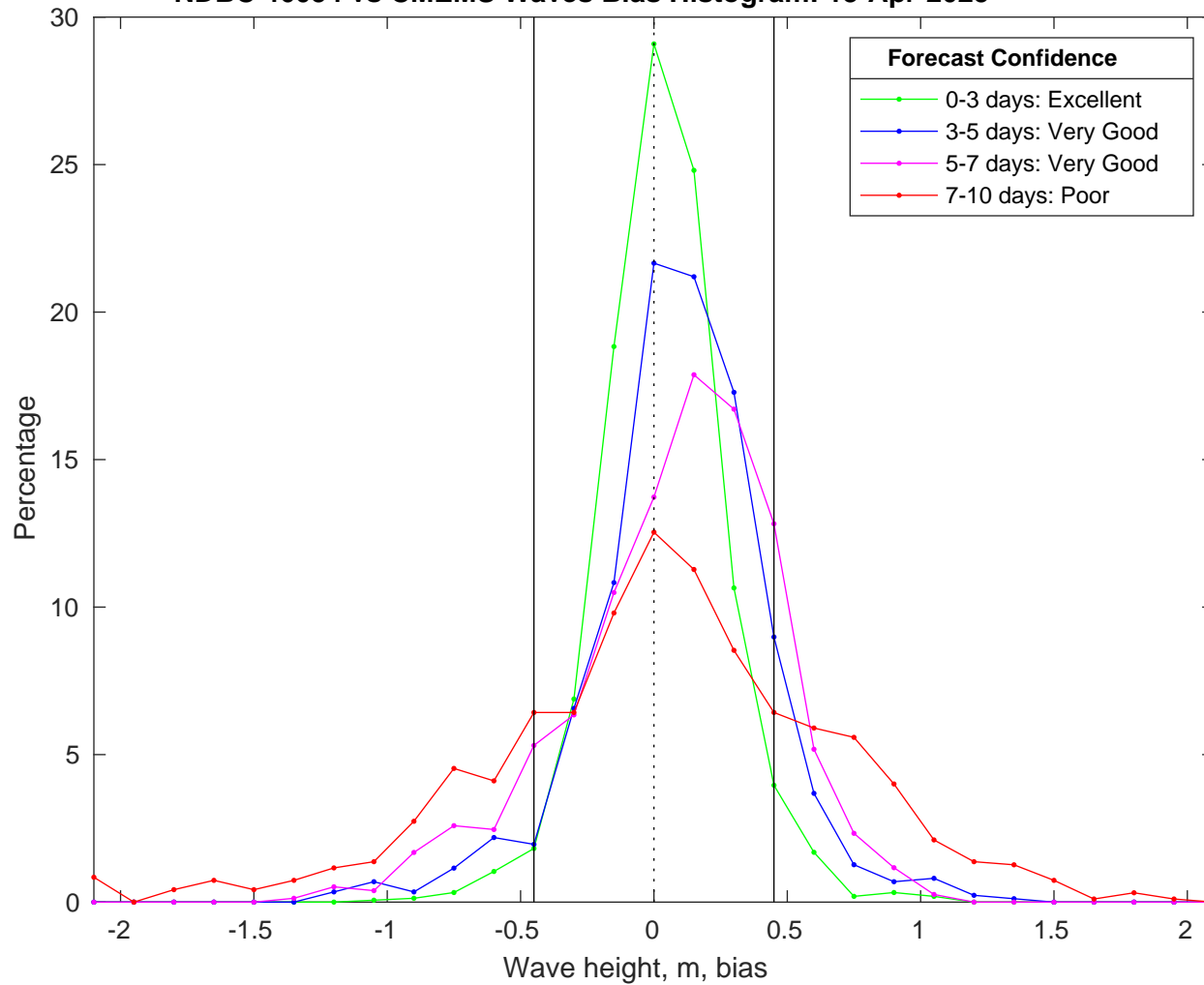
NDBC 46054 vs CMEMS Waves Bias Histogram: 13-Apr-2025
