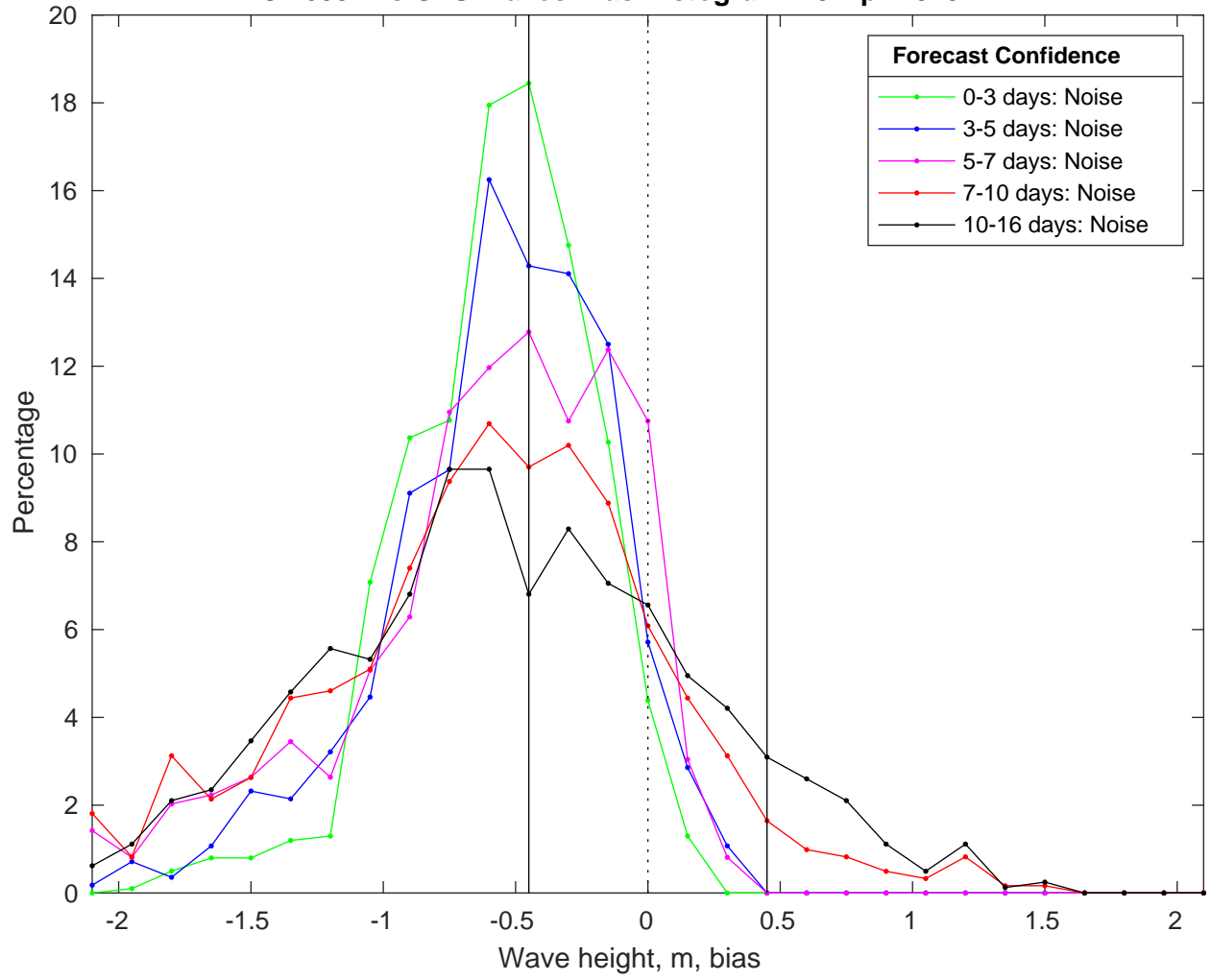
NDBC 46054 vs GFS Waves Bias Histogram: 13-Apr-2025
