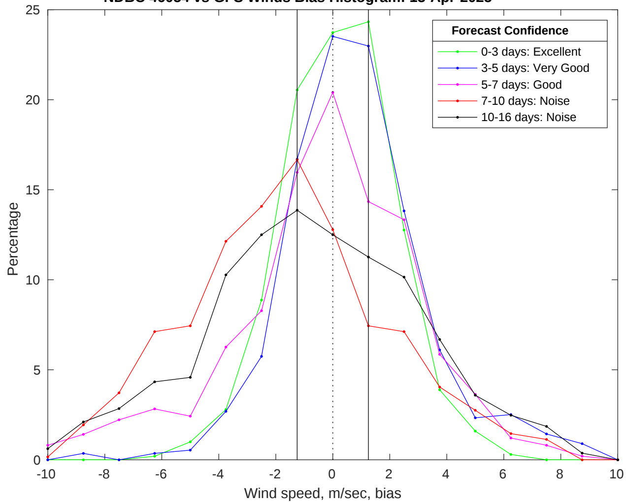
NDBC 46054 vs GFS Winds Bias Histogram: 13-Apr-2025
