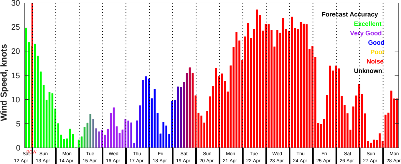
GFS Wind Speed Forecast for NDBC 46054 from 12-Apr-2025 16:00:00 to 28-Apr-2025 16:00:00
