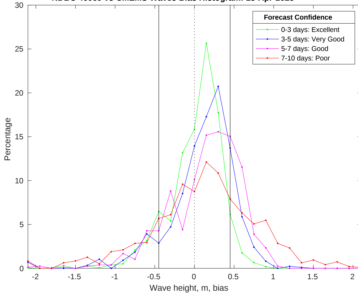
NDBC 46069 vs CMEMS Waves Bias Histogram: 13-Apr-2025
