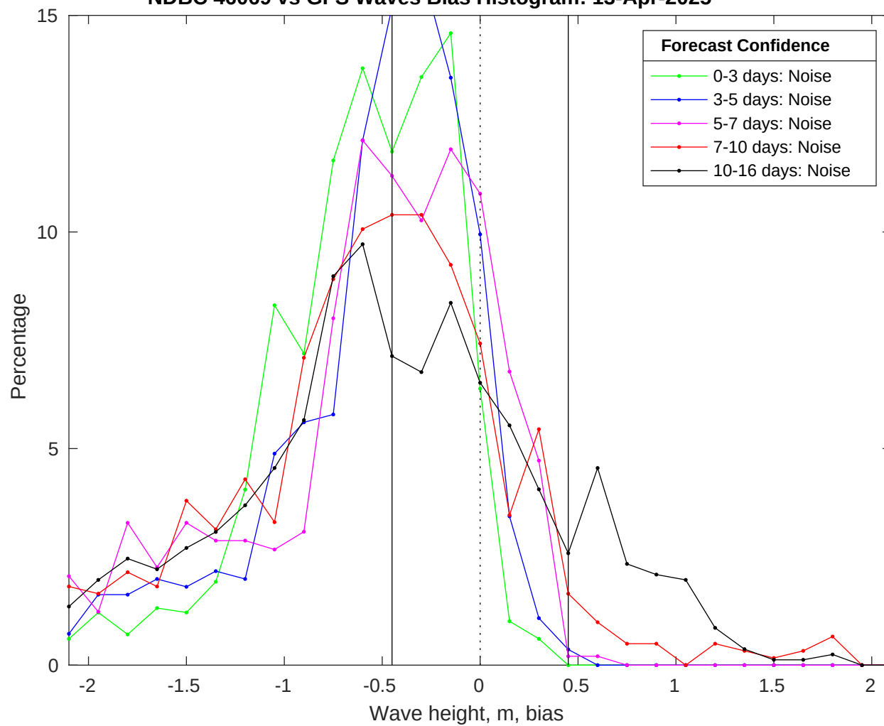
NDBC 46069 vs GFS Waves Bias Histogram: 13-Apr-2025
