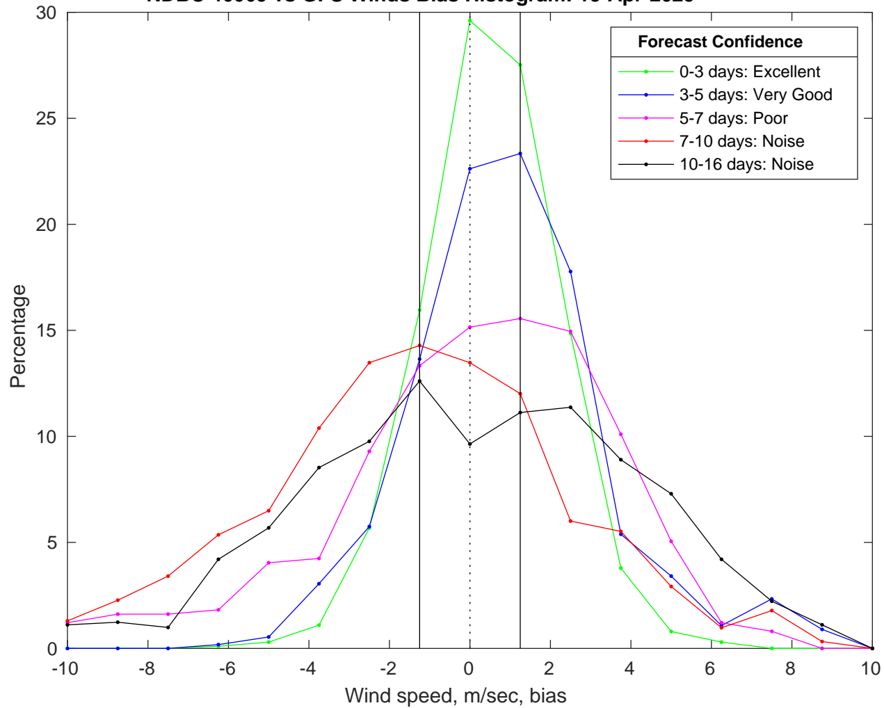
NDBC 46069 vs GFS Winds Bias Histogram: 13-Apr-2025
