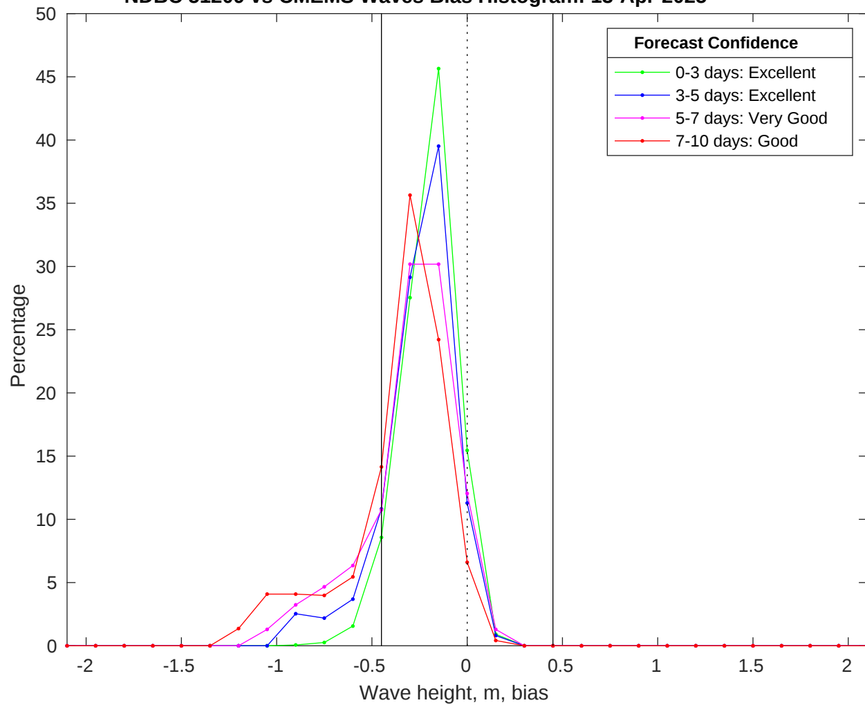
NDBC 51209 vs CMEMS Waves Bias Histogram: 13-Apr-2025
