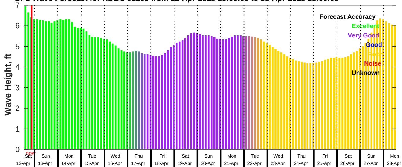
GFS Wave Forecast for NDBC 51209 from 12-Apr-2025 13:00:00 to 28-Apr-2025 13:00:00
