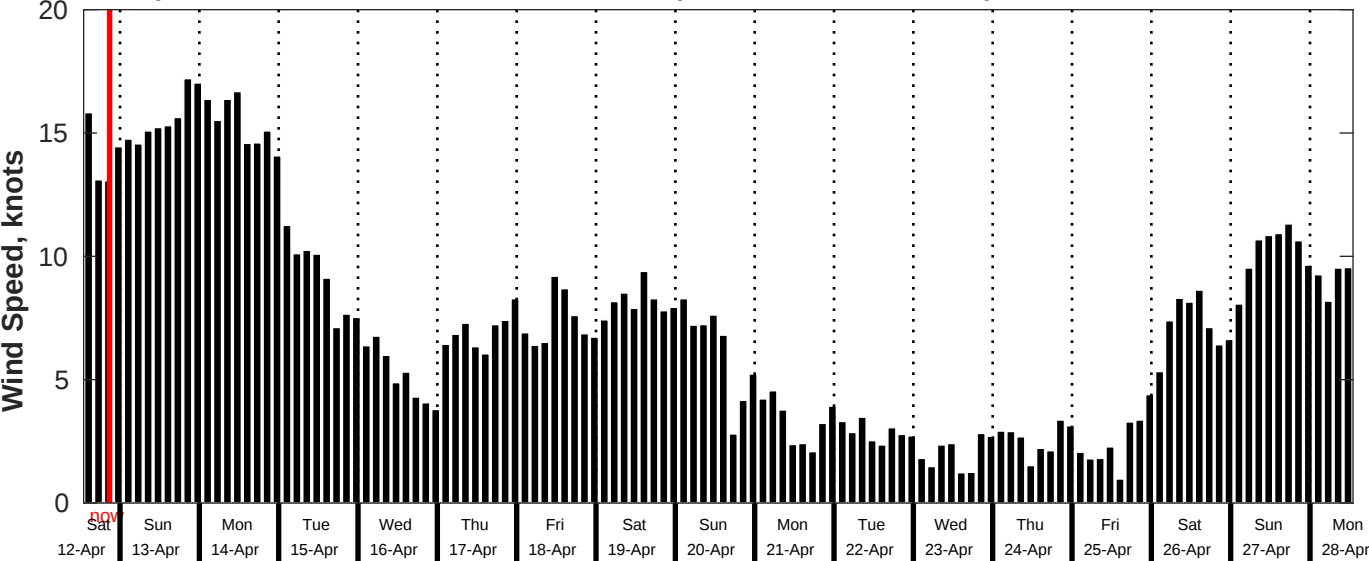
GFS Wind Speed Forecast for NDBC 51209 from 12-Apr-2025 13:00:00 to 28-Apr-2025 13:00:00
