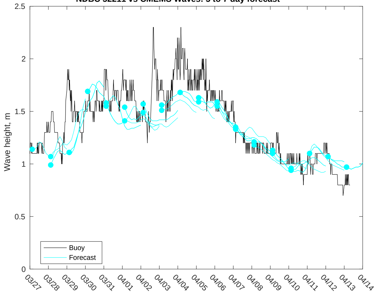
NDBC 52211 vs CMEMS Waves: 5 to 7 day forecast
