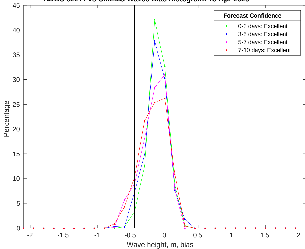
NDBC 52211 vs CMEMS Waves Bias Histogram: 13-Apr-2025
