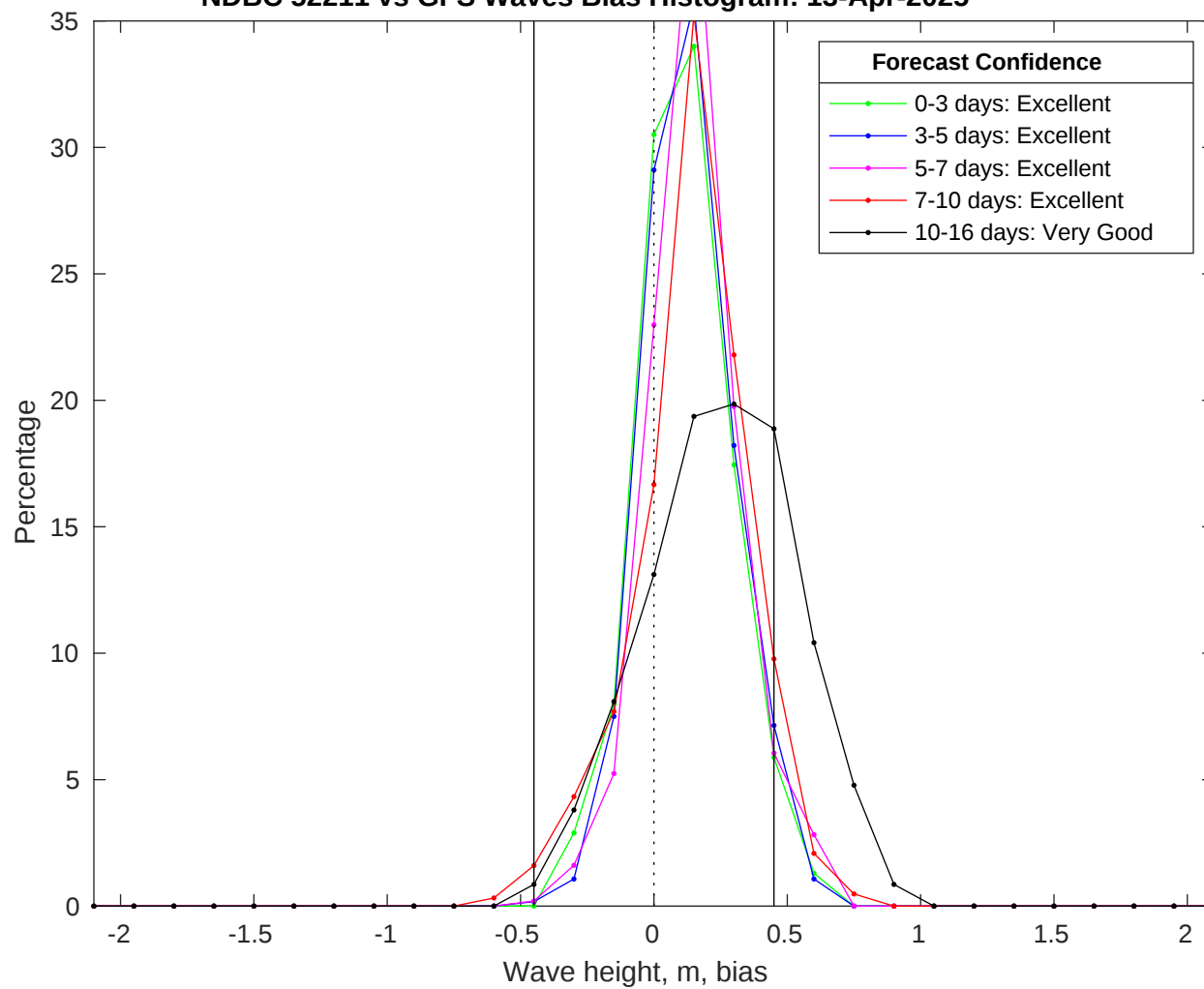
NDBC 52211 vs GFS Waves Bias Histogram: 13-Apr-2025
