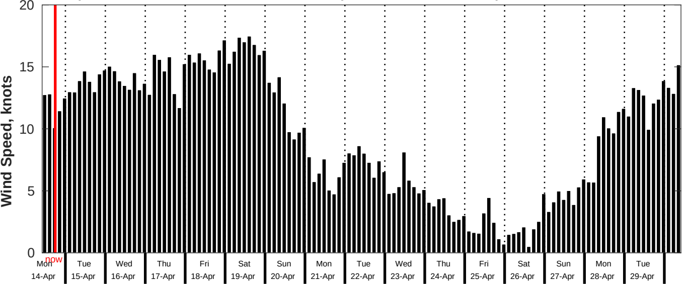
GFS Wind Speed Forecast for NDBC 52211 from 13-Apr-2025 10:00:00 to 29-Apr-2025 10:00:00
