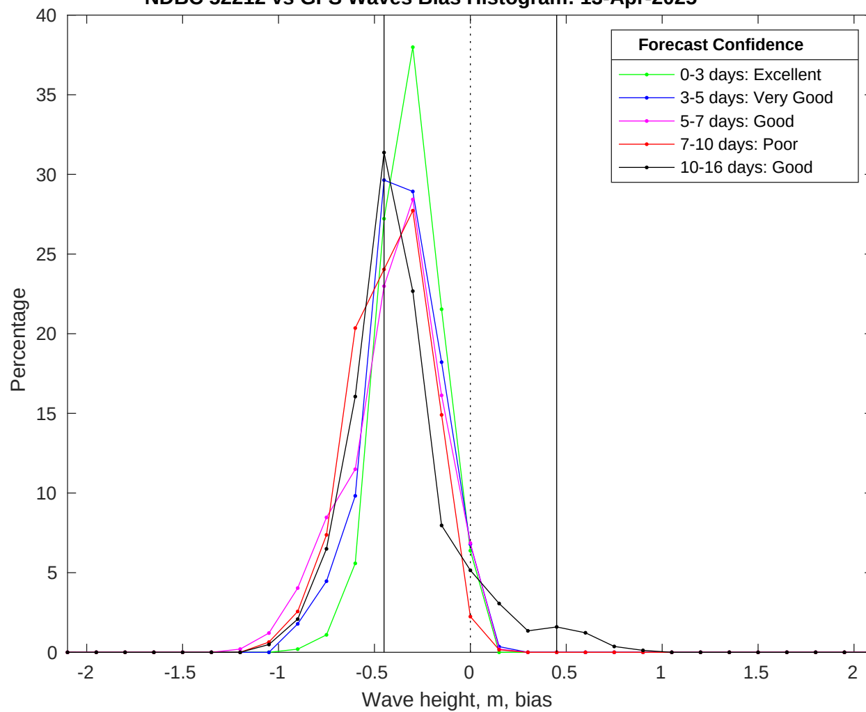
NDBC 52212 vs GFS Waves Bias Histogram: 13-Apr-2025
