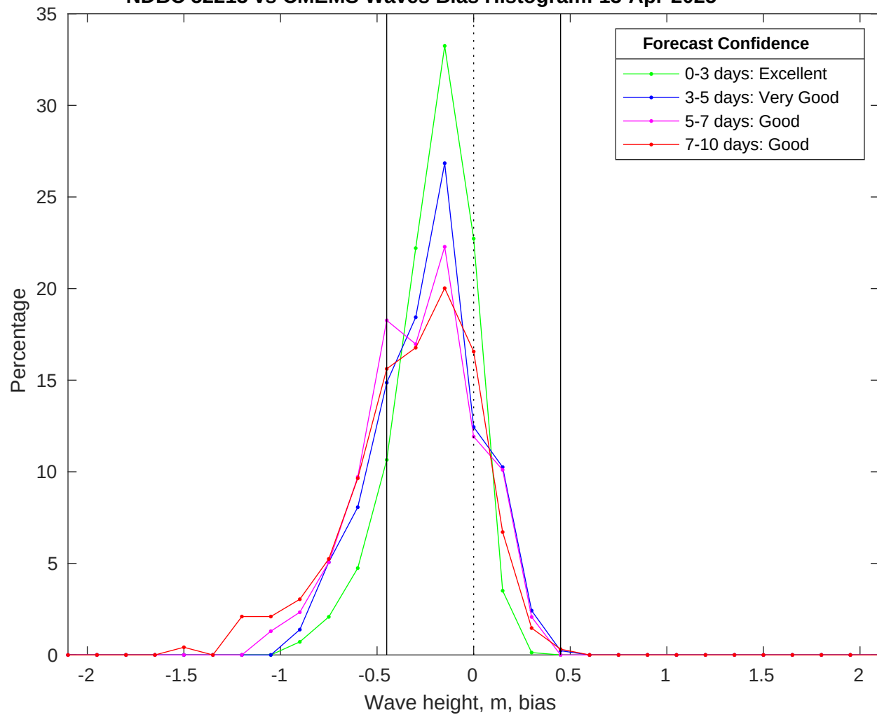
NDBC 52213 vs CMEMS Waves Bias Histogram: 13-Apr-2025
