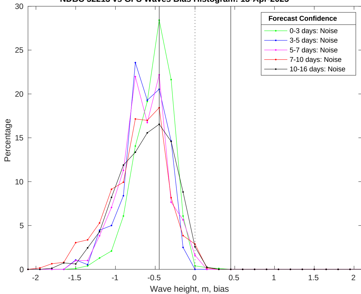
NDBC 52213 vs GFS Waves Bias Histogram: 13-Apr-2025
