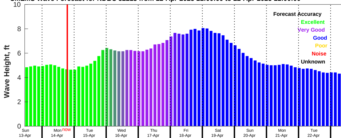
CMEMS Wave Forecast for NDBC 52213 from 12-Apr-2025 11:00:00 to 22-Apr-2025 11:00:00
