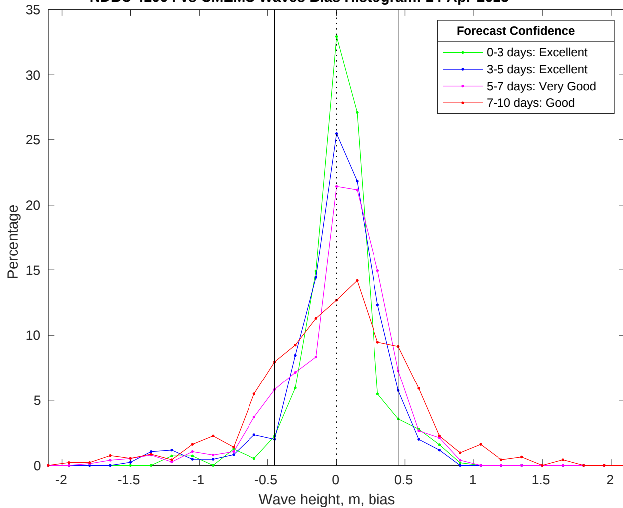
NDBC 41004 vs CMEMS Waves Bias Histogram: 14-Apr-2025
