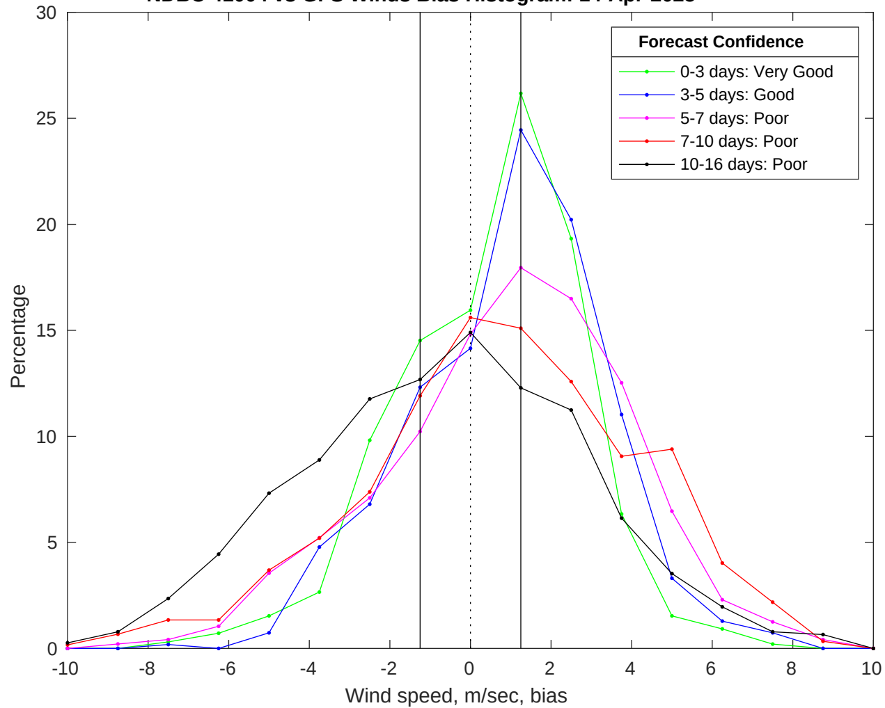
NDBC 41004 vs GFS Winds Bias Histogram: 14-Apr-2025
