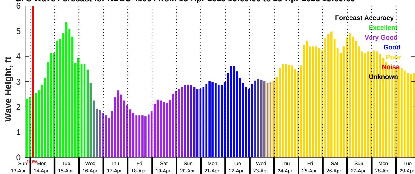
GFS Wave Forecast for NDBC 41004 from 13-Apr-2025 19:00:00 to 29-Apr-2025 19:00:00
