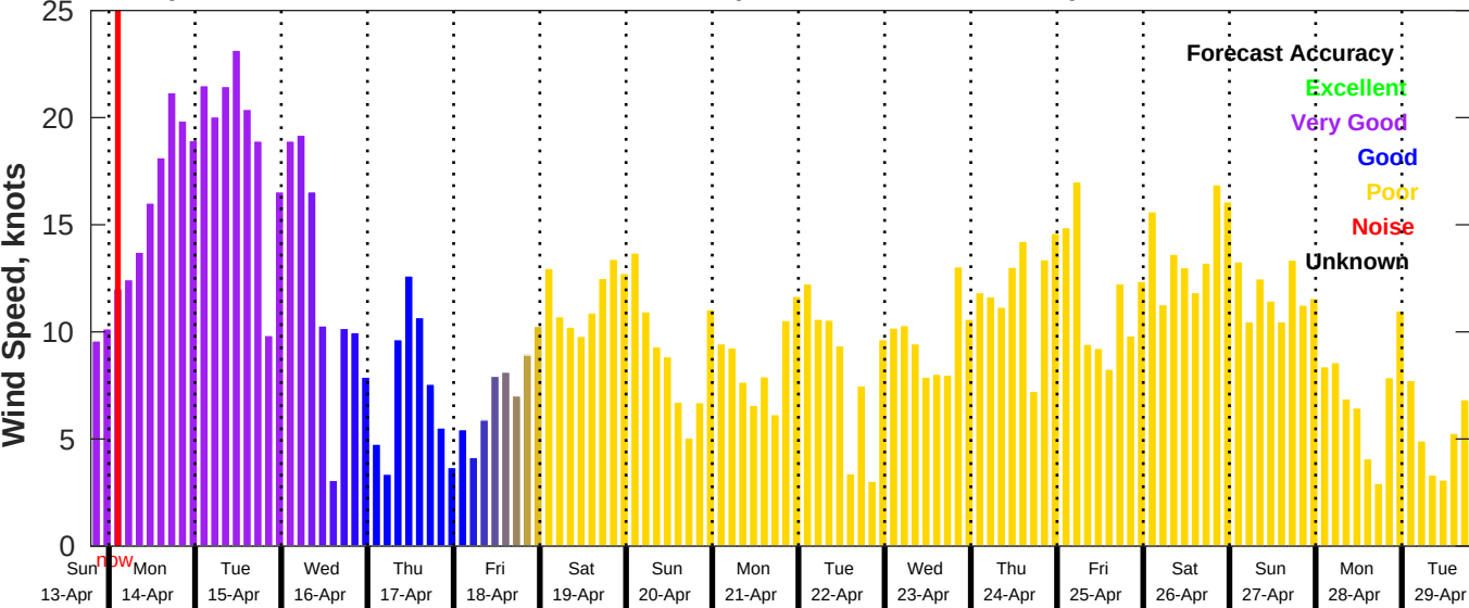
GFS Wind Speed Forecast for NDBC 41004 from 13-Apr-2025 19:00:00 to 29-Apr-2025 19:00:00
