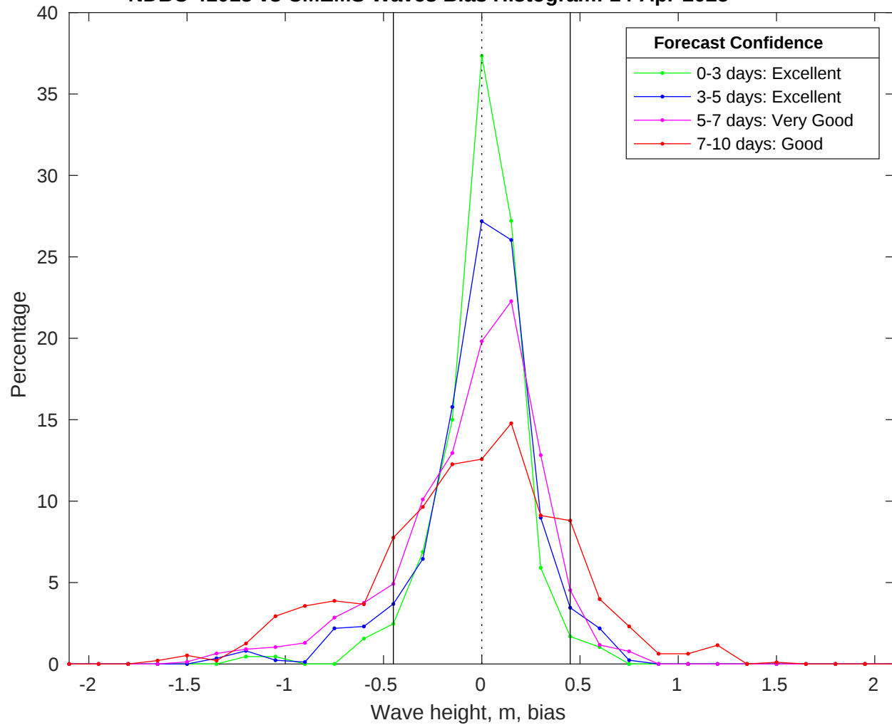
NDBC 41013 vs CMEMS Waves Bias Histogram: 14-Apr-2025
