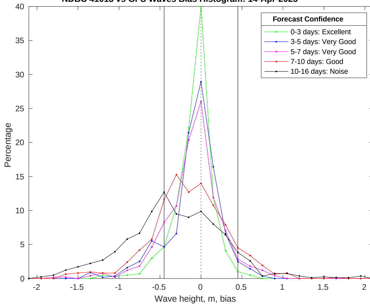
NDBC 41013 vs GFS Waves Bias Histogram: 14-Apr-2025
