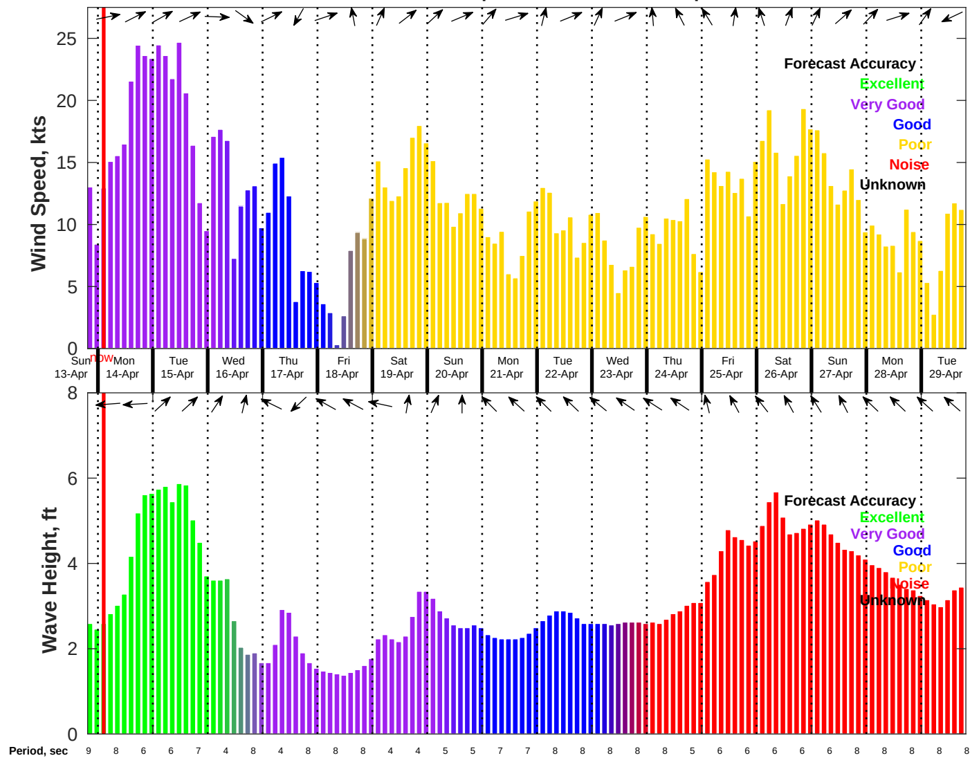
Wind & Wave Forecast for NDBC 41013 from 13-Apr-2025 19:00:00 to 29-Apr-2025 19:00:00
