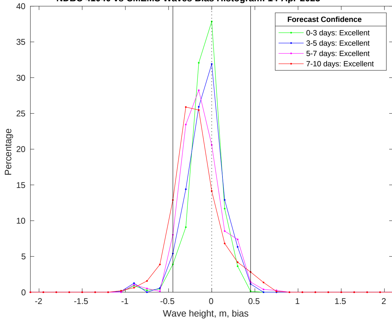
NDBC 41040 vs CMEMS Waves Bias Histogram: 14-Apr-2025
