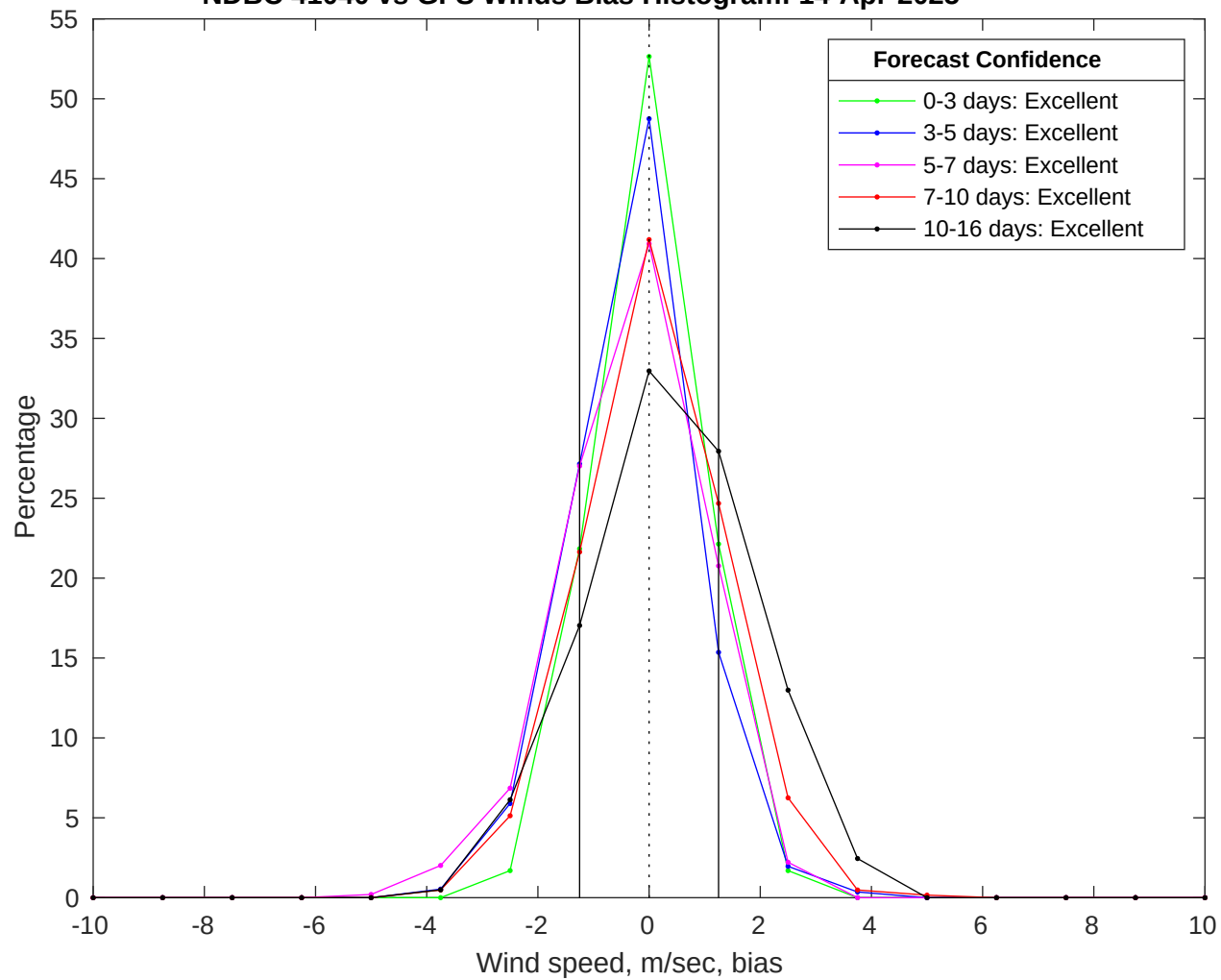
NDBC 41040 vs GFS Winds Bias Histogram: 14-Apr-2025
