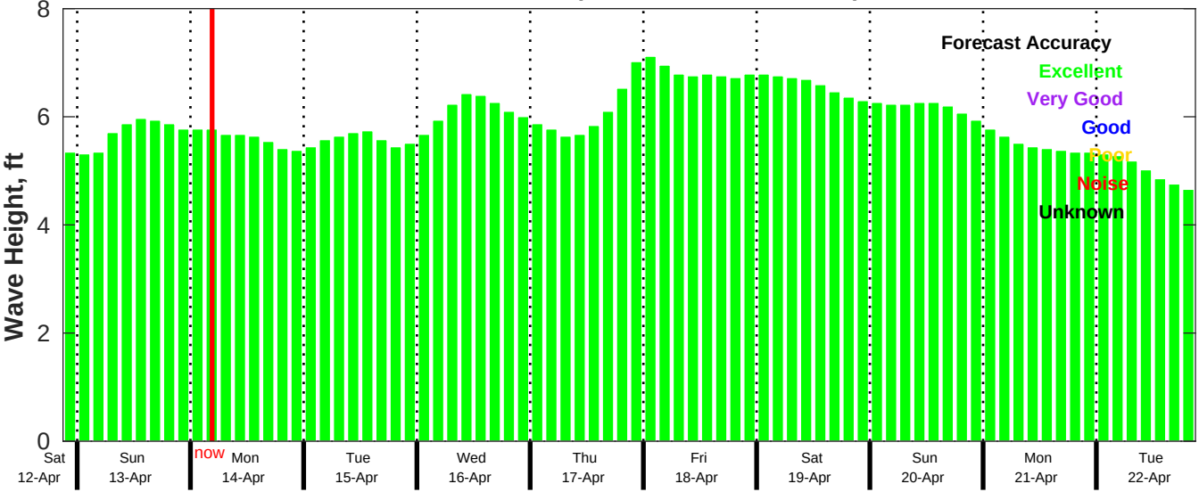
CMEMS Wave Forecast for NDBC 41040 from 12-Apr-2025 21:00:00 to 22-Apr-2025 21:00:00
