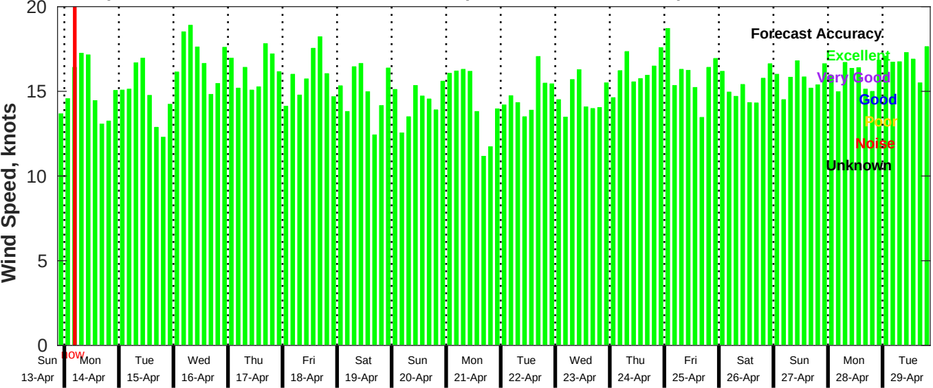
GFS Wind Speed Forecast for NDBC 41040 from 13-Apr-2025 21:00:00 to 29-Apr-2025 21:00:00
