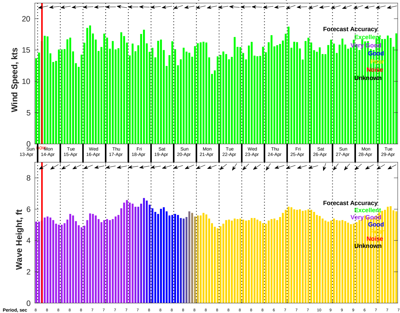
Wind & Wave Forecast for NDBC 41040 from 13-Apr-2025 21:00:00 to 29-Apr-2025 21:00:00
