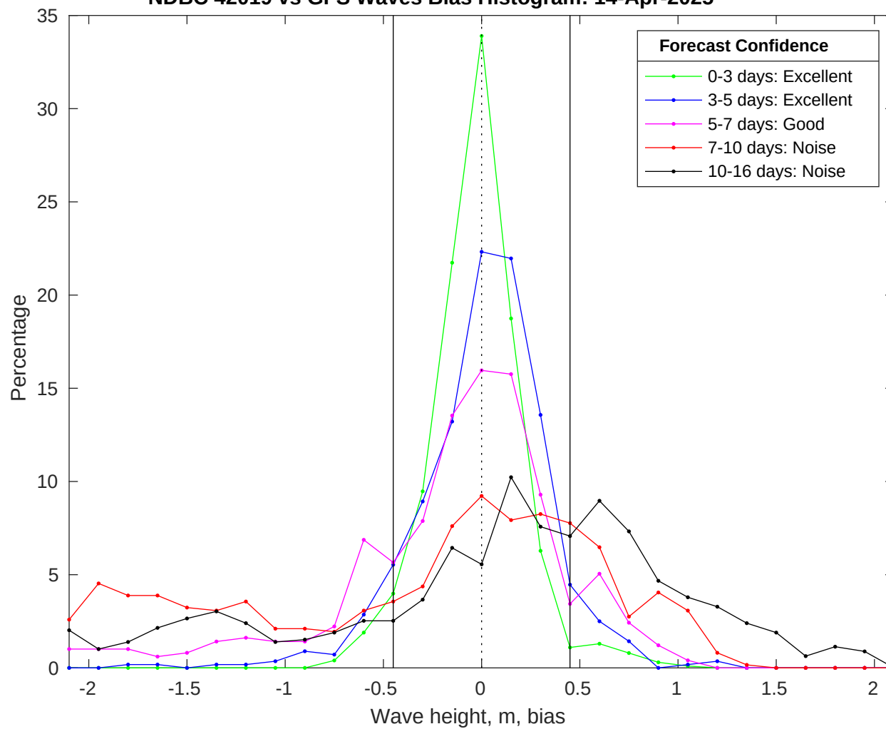
NDBC 42019 vs GFS Waves Bias Histogram: 14-Apr-2025
