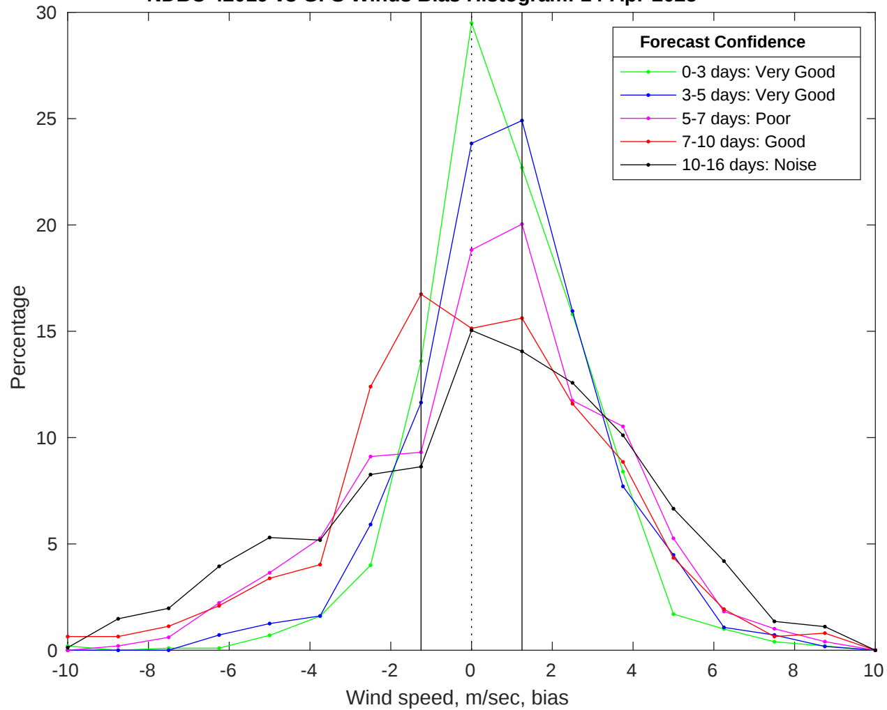
NDBC 42019 vs GFS Winds Bias Histogram: 14-Apr-2025
