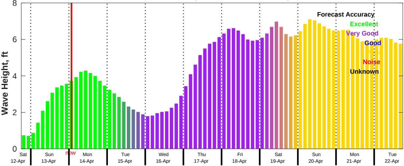
CMEMS Wave Forecast for NDBC 42019 from 12-Apr-2025 18:00:00 to 22-Apr-2025 18:00:00
