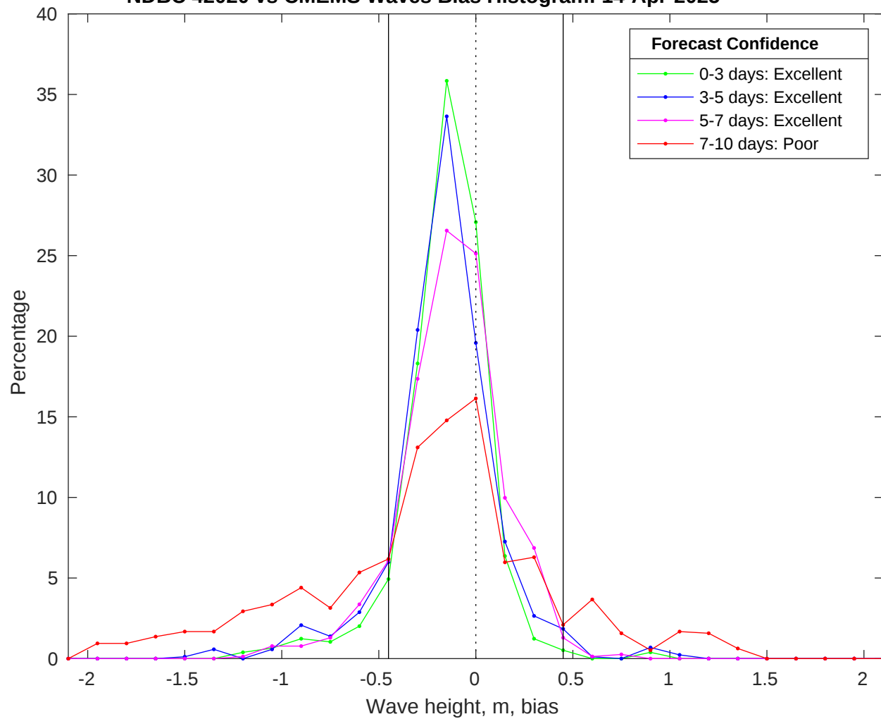
NDBC 42020 vs CMEMS Waves Bias Histogram: 14-Apr-2025
