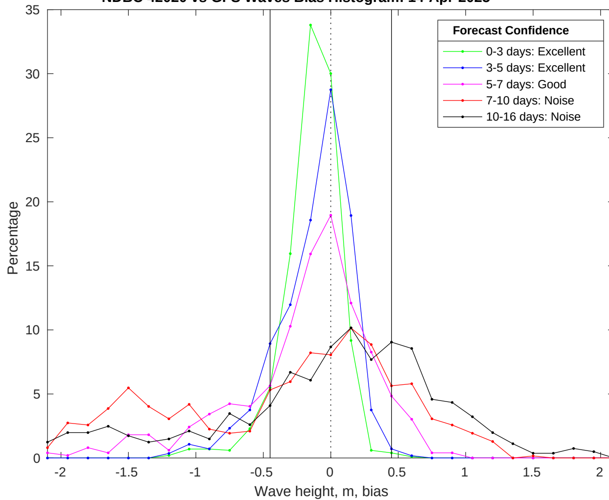
NDBC 42020 vs GFS Waves Bias Histogram: 14-Apr-2025
