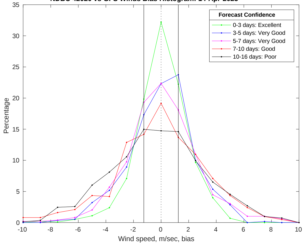
NDBC 42020 vs GFS Winds Bias Histogram: 14-Apr-2025
