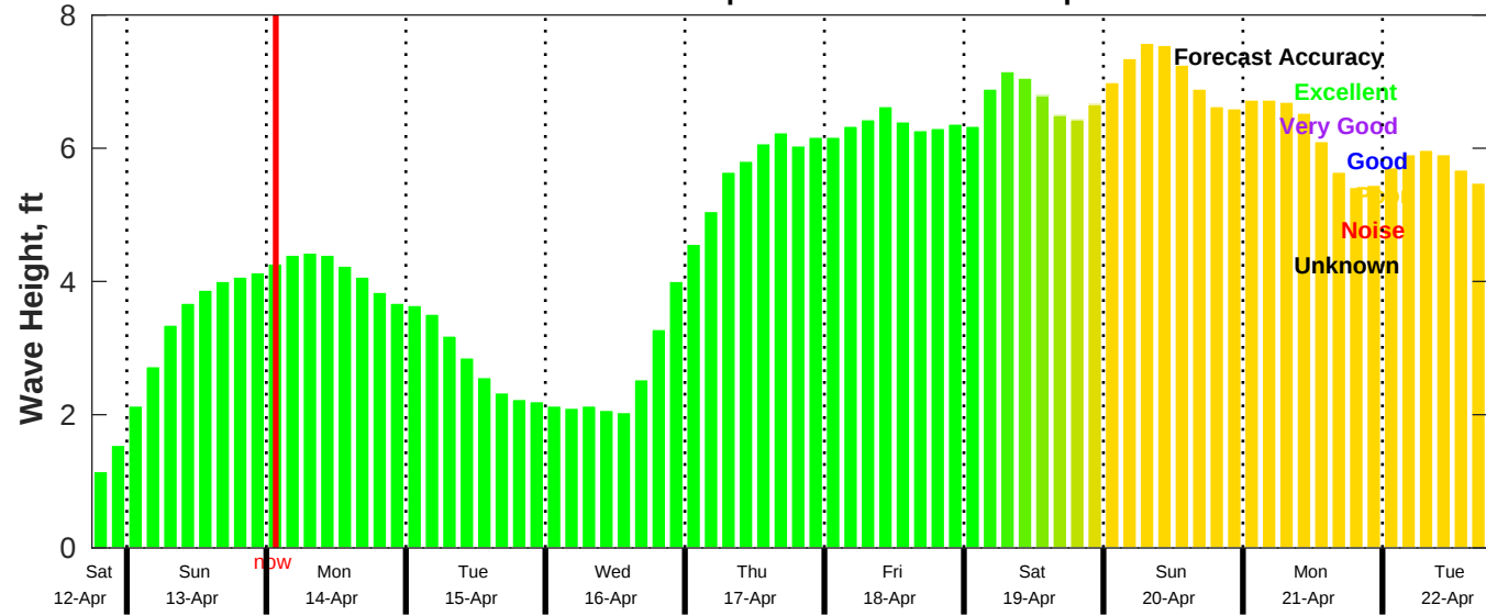
CMEMS Wave Forecast for NDBC 42020 from 12-Apr-2025 18:00:00 to 22-Apr-2025 18:00:00
