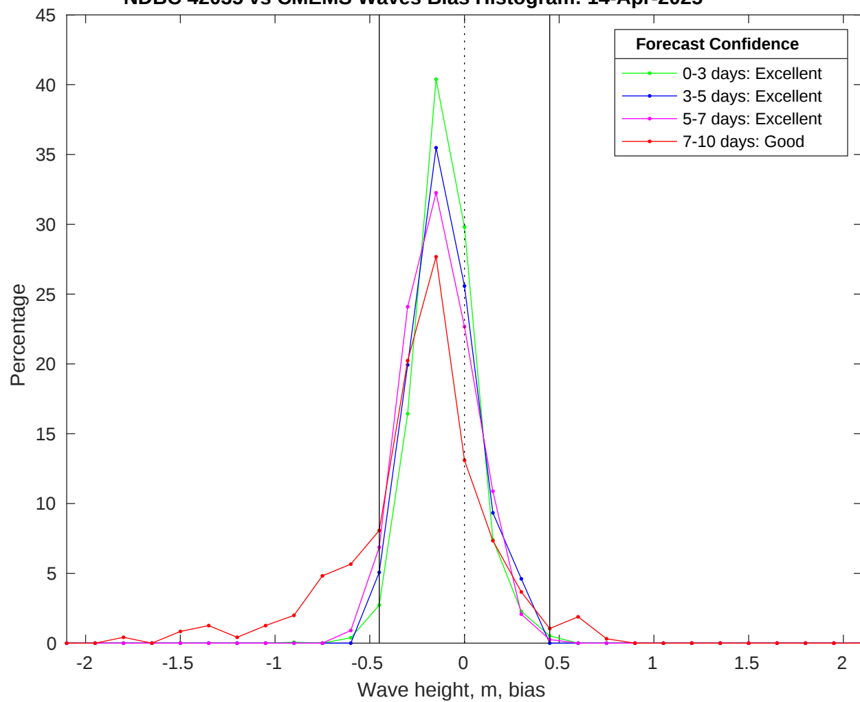
NDBC 42035 vs CMEMS Waves Bias Histogram: 14-Apr-2025
