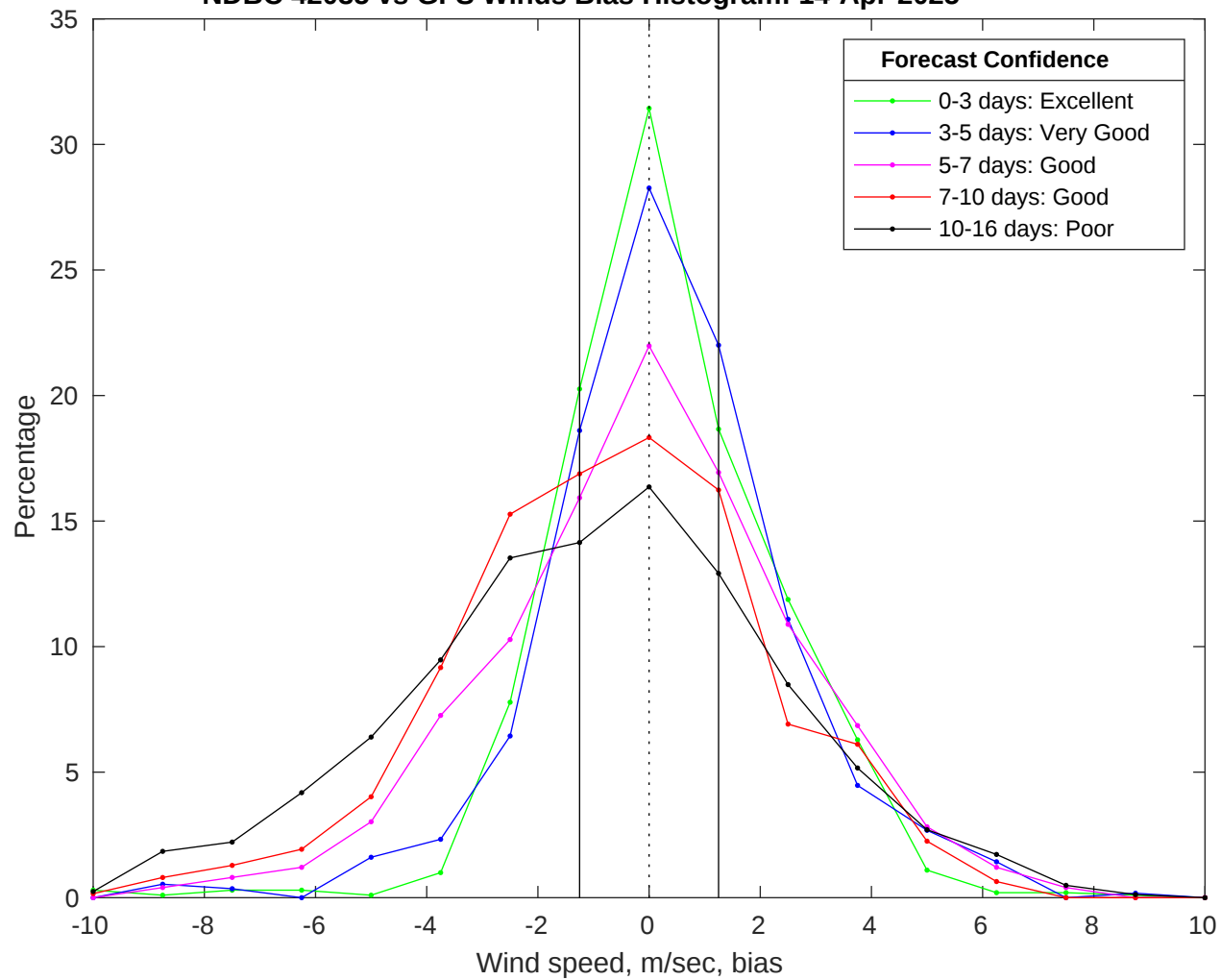
NDBC 42035 vs GFS Winds Bias Histogram: 14-Apr-2025
