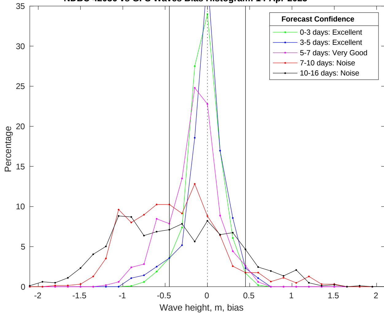
NDBC 42036 vs GFS Waves Bias Histogram: 14-Apr-2025
