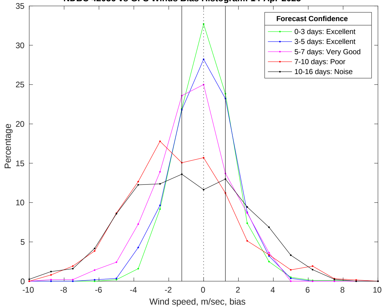
NDBC 42036 vs GFS Winds Bias Histogram: 14-Apr-2025
